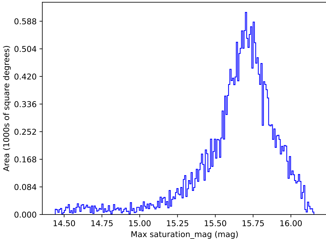
all_long_v3.4_10yrs All sky r band: Max saturation_mag
