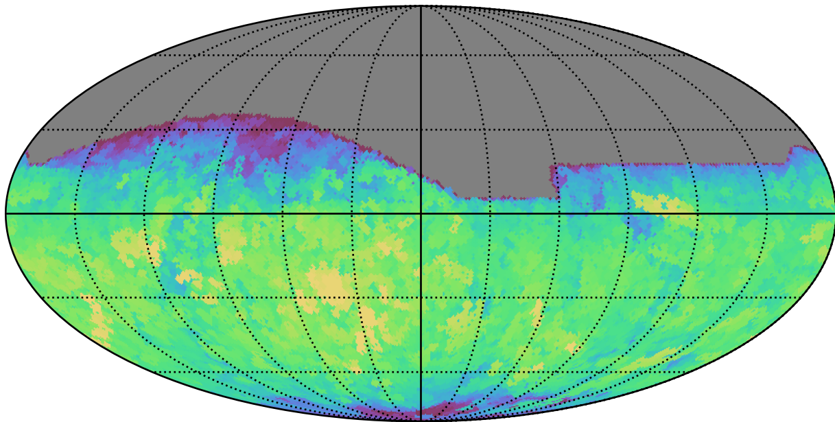
all_long_v3.4_10yrs All sky i band: Max saturation_mag
