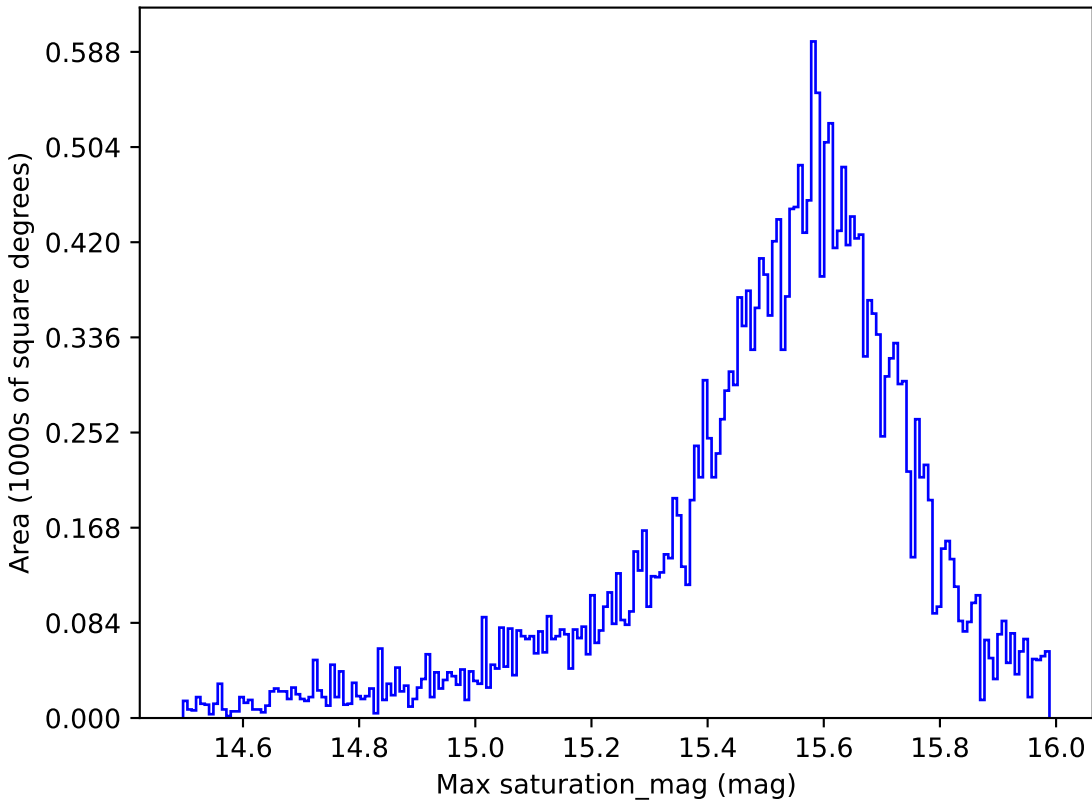
all_long_v3.4_10yrs All sky i band: Max saturation_mag
