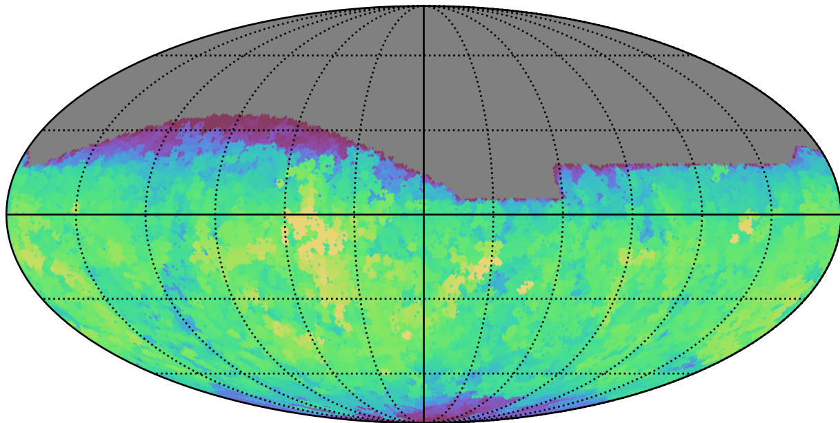
all_long_v3.4_10yrs All sky g band: Max saturation_mag
