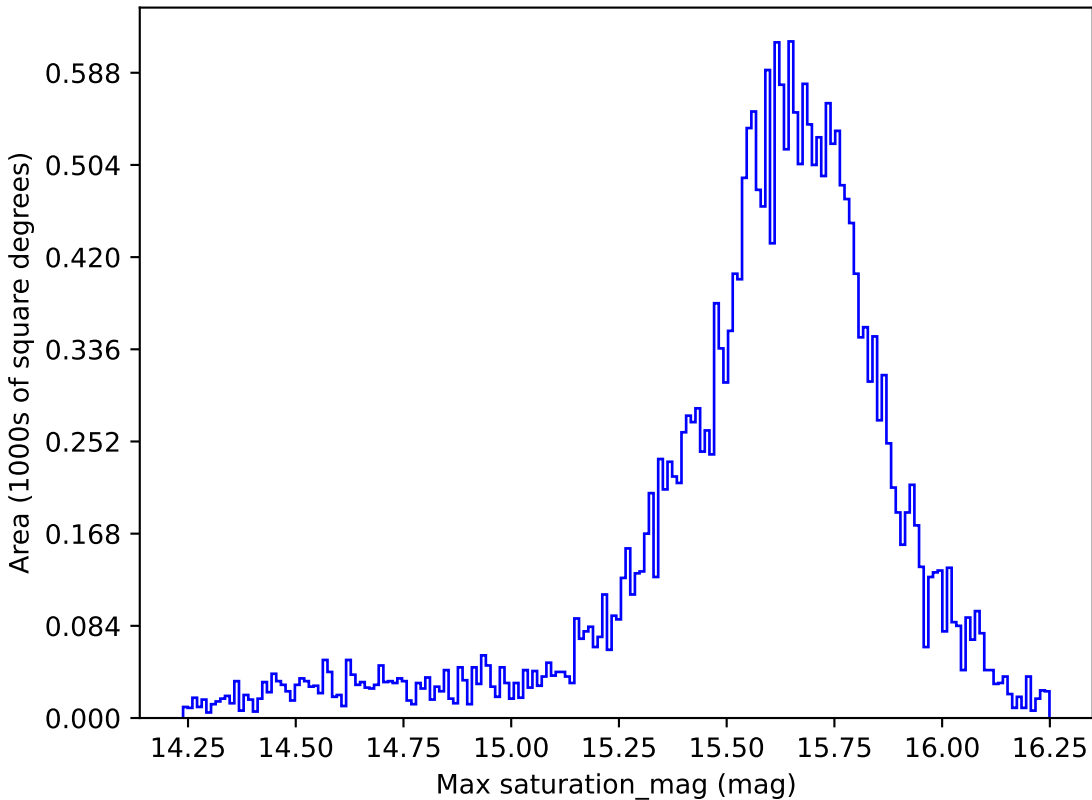
all_long_v3.4_10yrs All sky g band: Max saturation_mag
