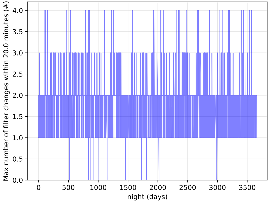
all_long_v3.4_10yrs Per Night: Max number of filter changes within 20.0 minutes
