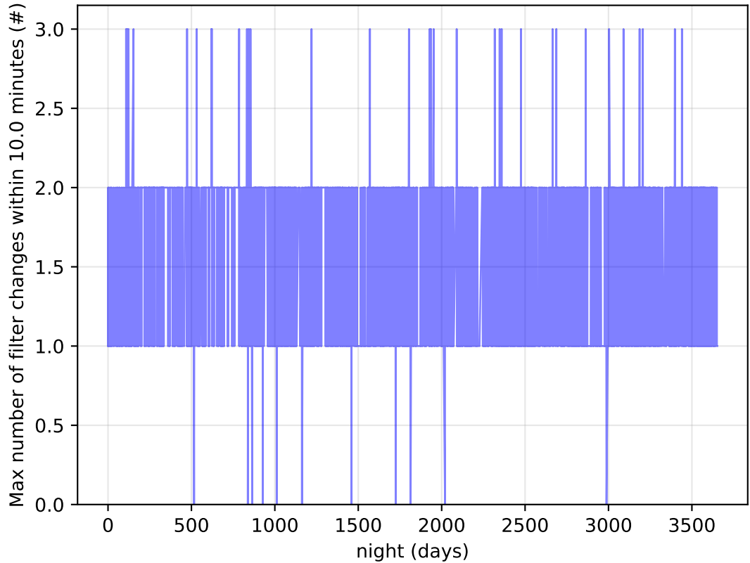
all_long_v3.4_10yrs Per Night: Max number of filter changes within 10.0 minutes
