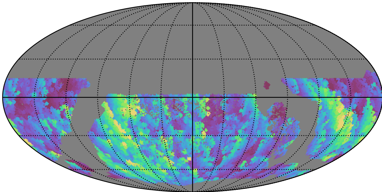
all_long_v3.4_10yrs WFD u band: Max normairmass
