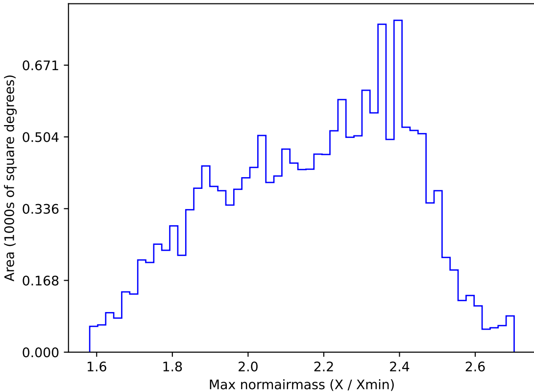
all_long_v3.4_10yrs WFD r band: Max normairmass
