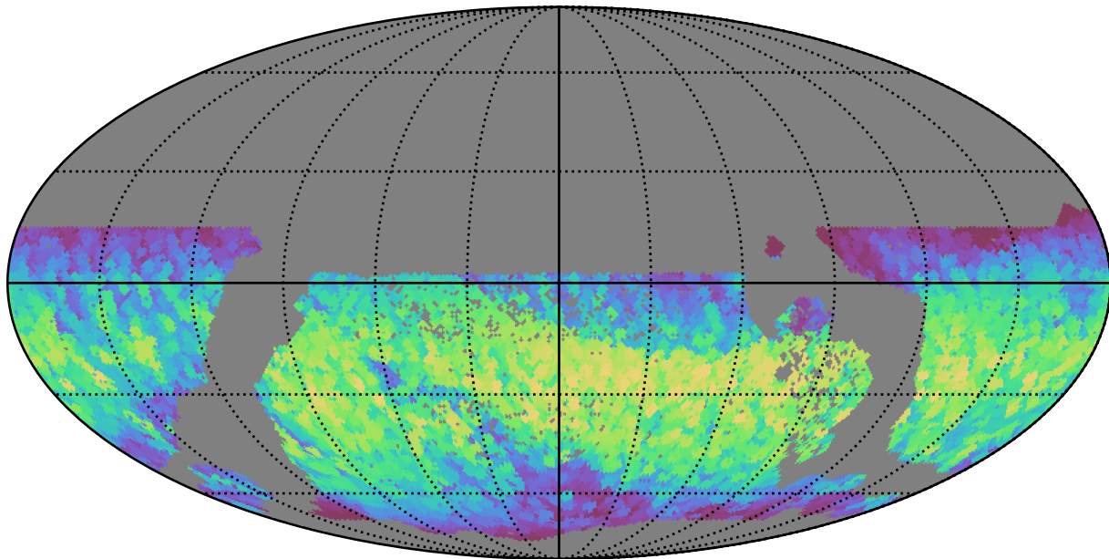
all_long_v3.4_10yrs WFD all bands: Max normairmass
