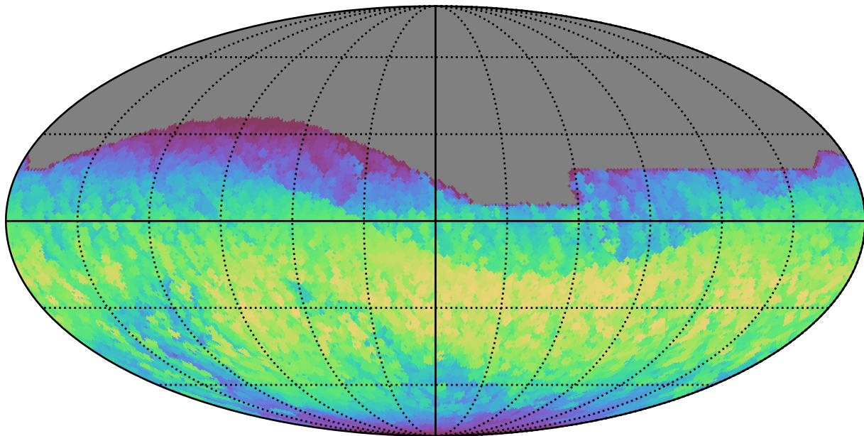
all_long_v3.4_10yrs All sky all bands: Max normairmass
