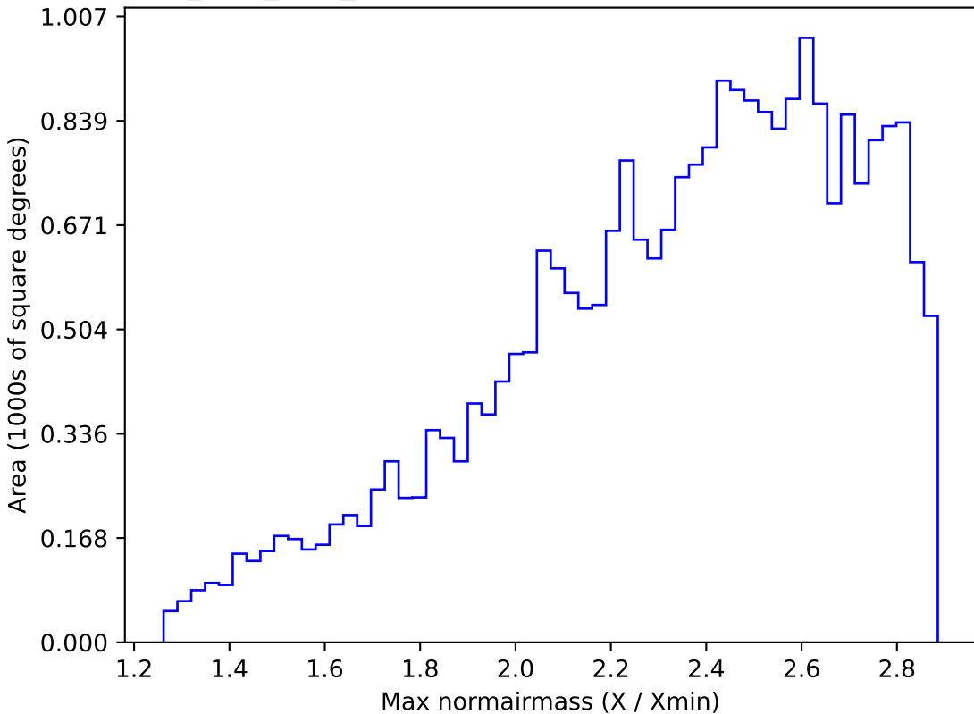
all_long_v3.4_10yrs All sky all bands: Max normairmass
