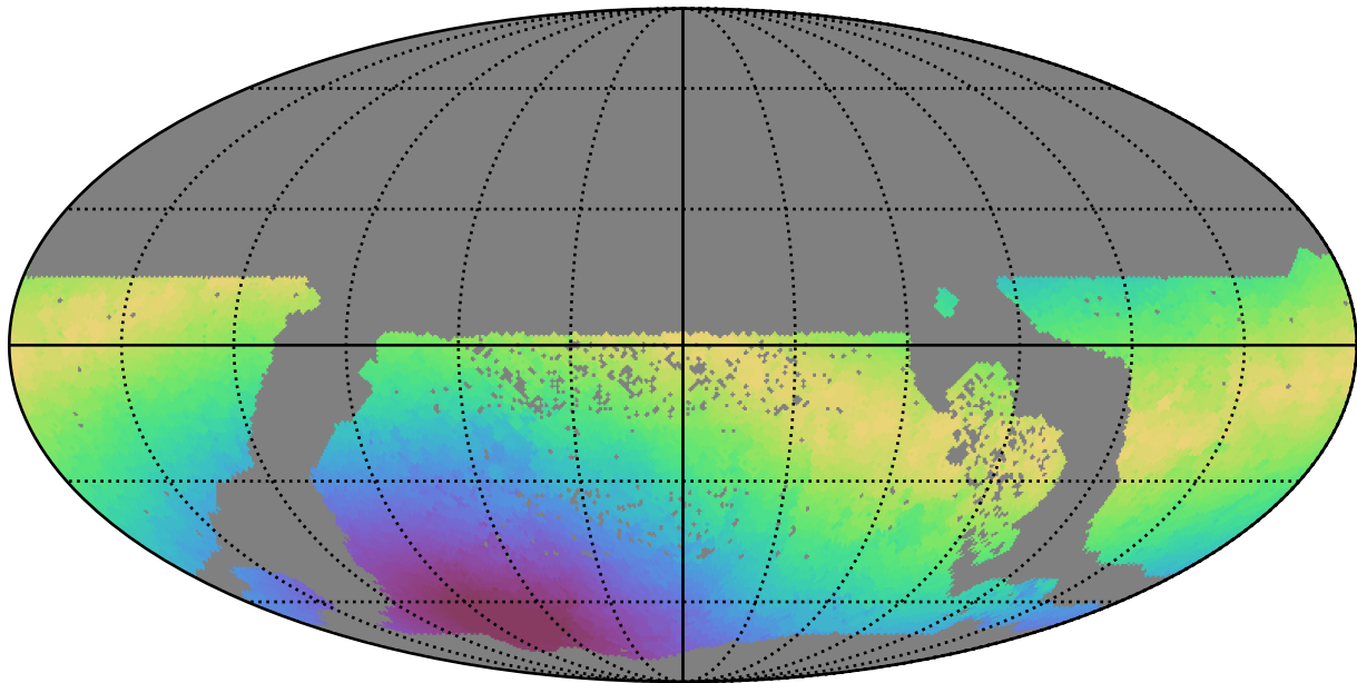
all_long_v3.4_10yrs WFD z band: Max moonDistance
