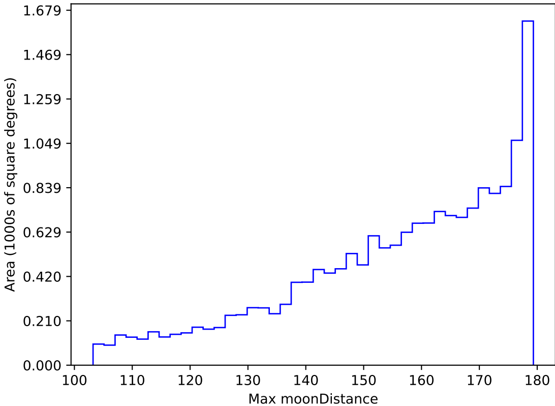
all_long_v3.4_10yrs WFD r band: Max moonDistance
