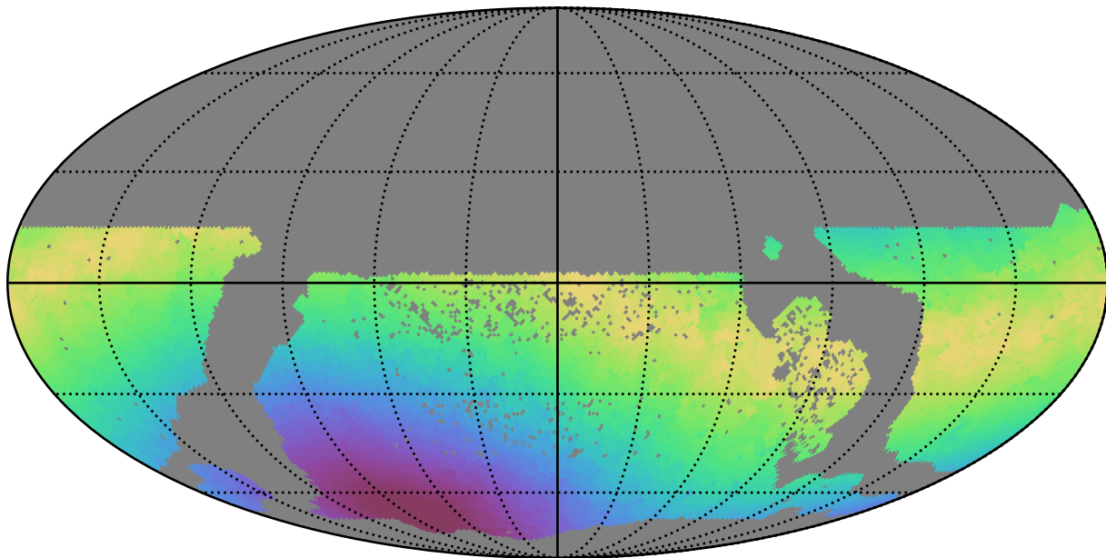
all_long_v3.4_10yrs WFD g band: Max moonDistance
