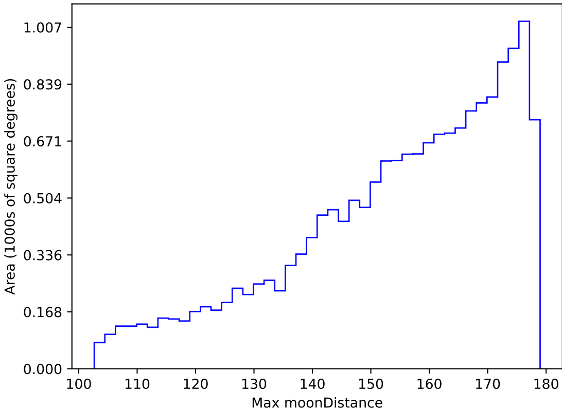
all_long_v3.4_10yrs WFD g band: Max moonDistance
