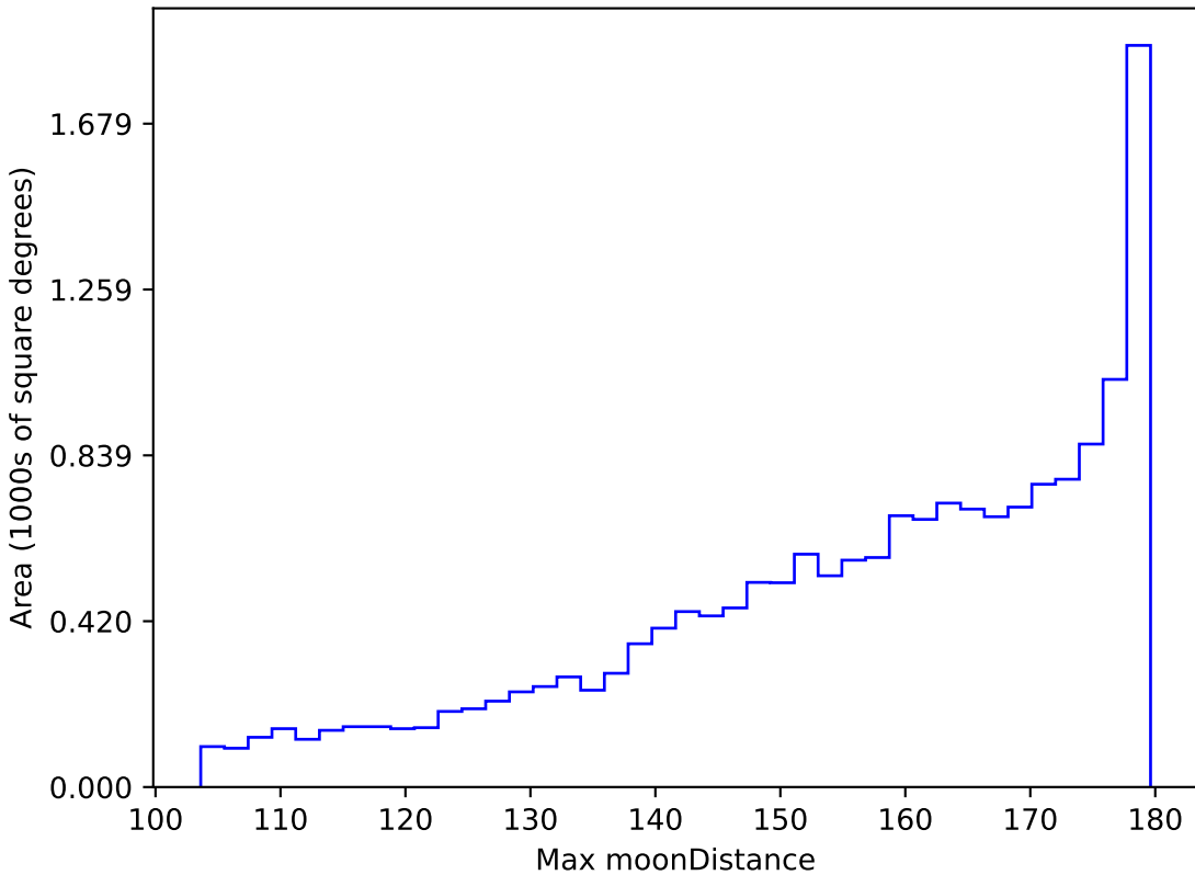
all_long_v3.4_10yrs WFD all bands: Max moonDistance
