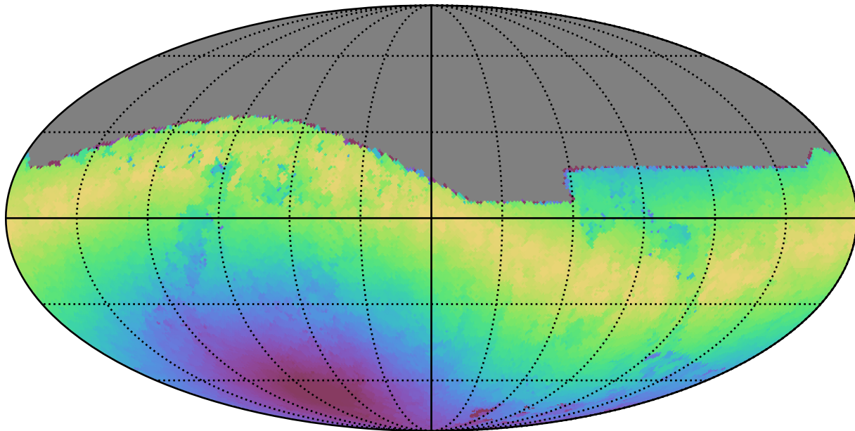
all_long_v3.4_10yrs All sky z band: Max moonDistance
