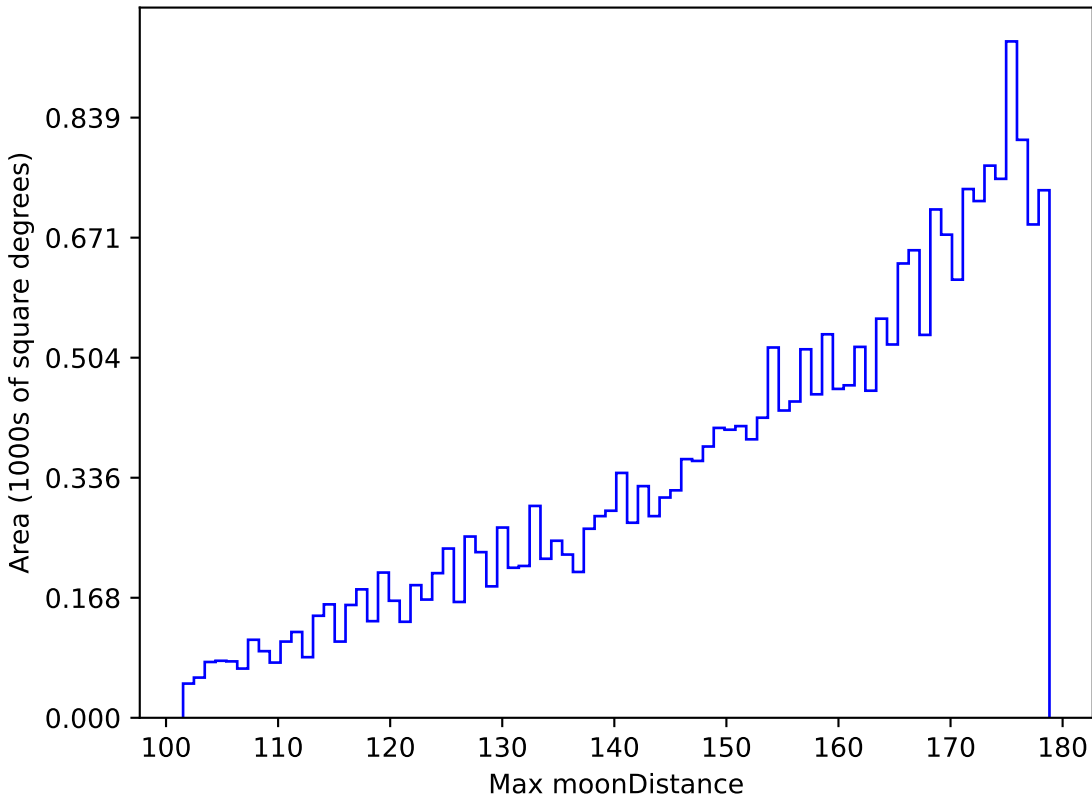
all_long_v3.4_10yrs All sky z band: Max moonDistance
