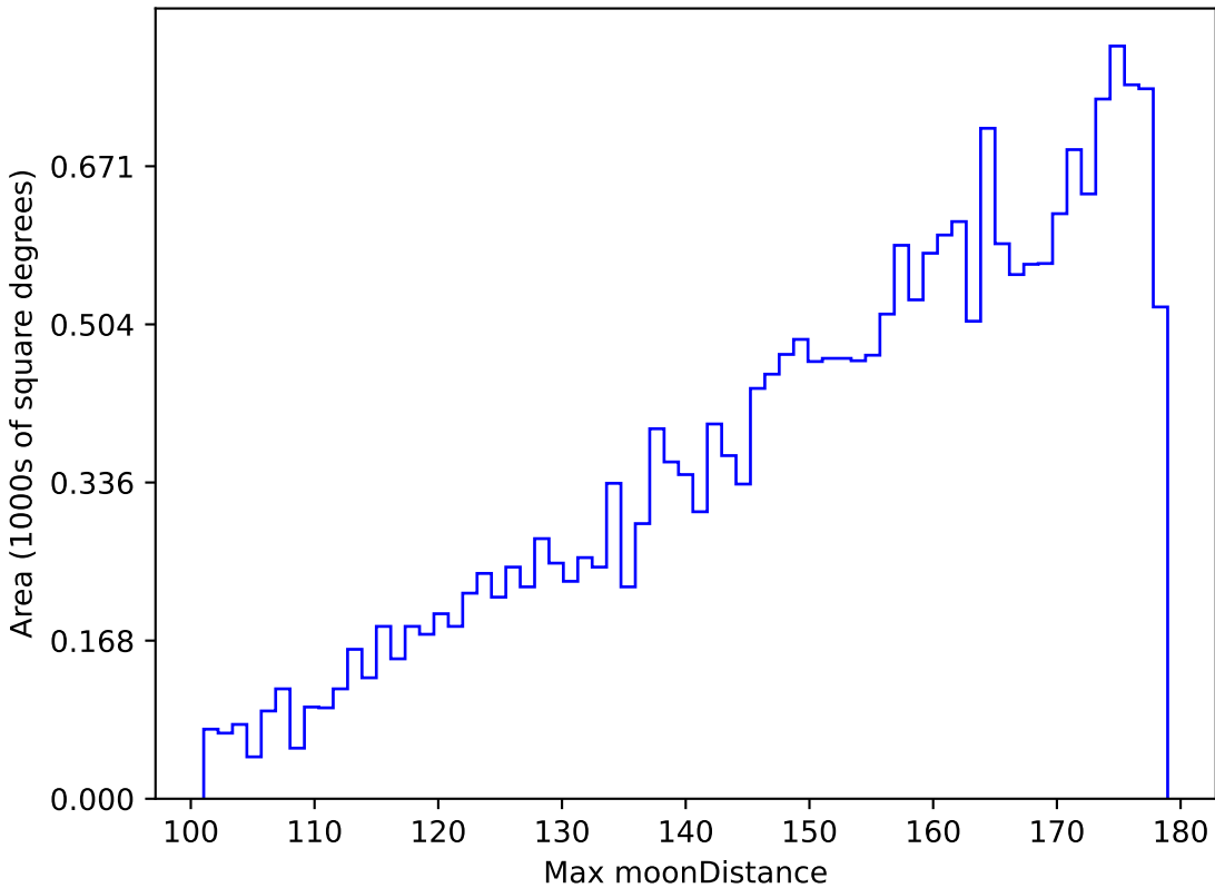
all_long_v3.4_10yrs All sky u band: Max moonDistance
