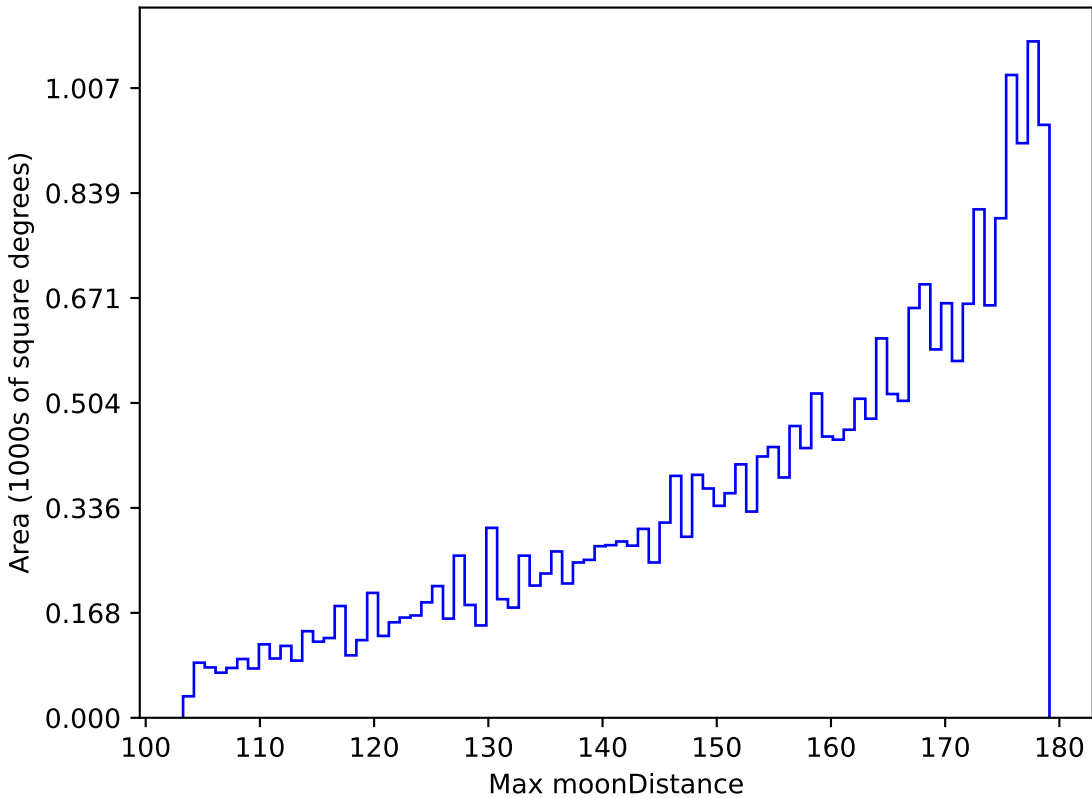
all_long_v3.4_10yrs All sky i band: Max moonDistance
