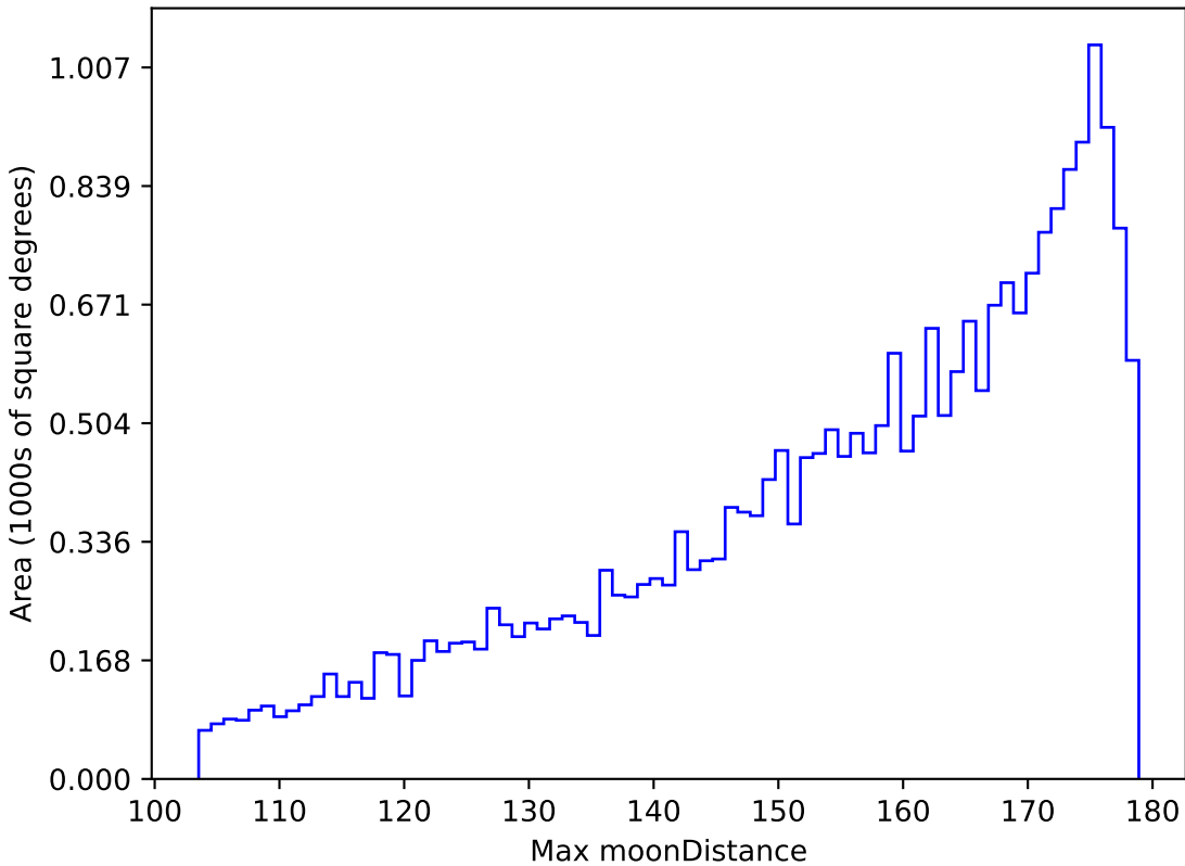
all_long_v3.4_10yrs All sky g band: Max moonDistance
