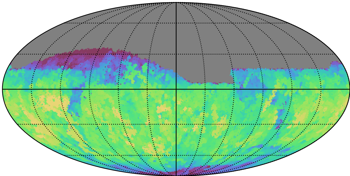
all_long_v3.4_10yrs Yr 1 z band: Max fiveSigmaDepth
