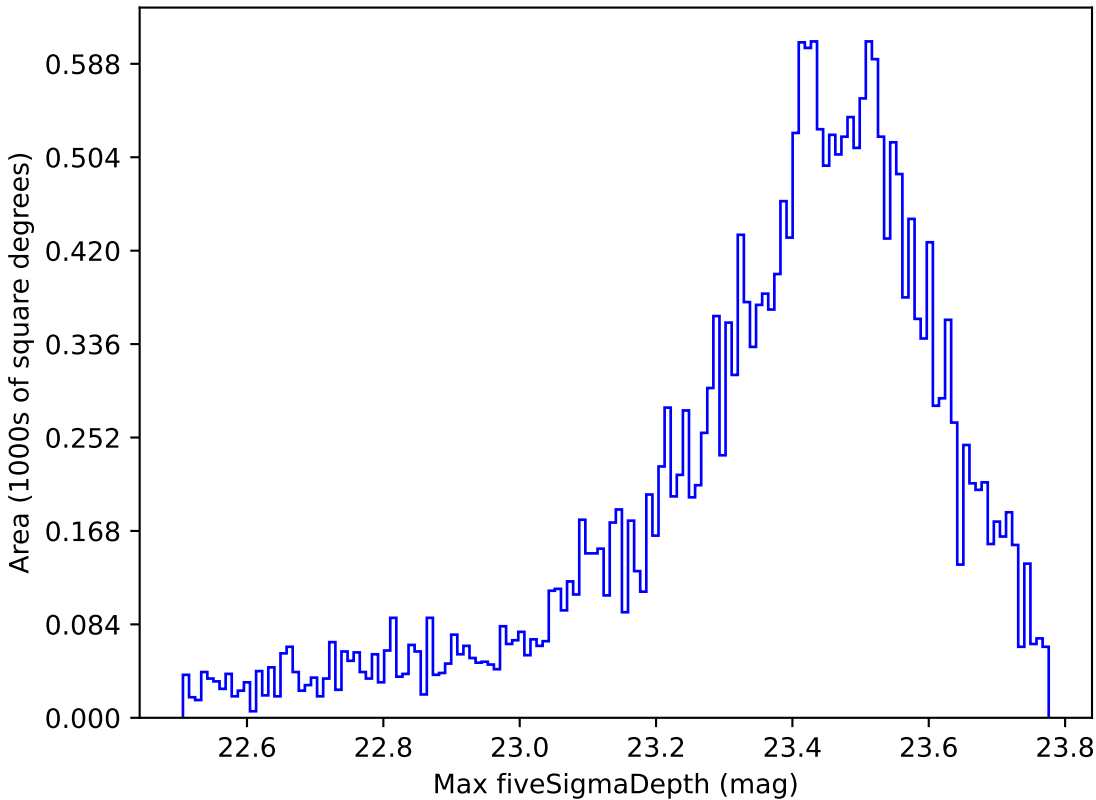
all_long_v3.4_10yrs Yr 1 z band: Max fiveSigmaDepth
