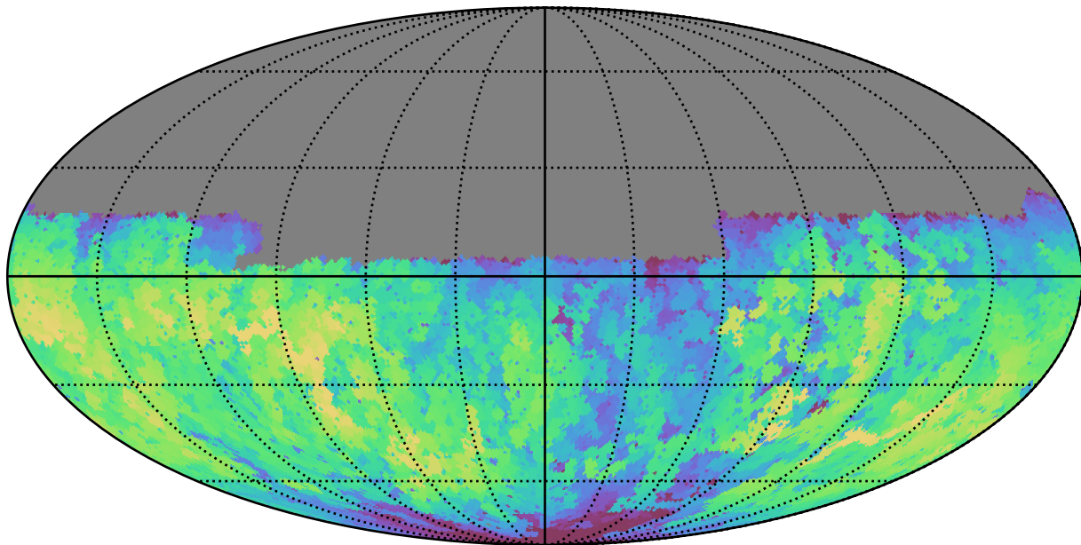
all_long_v3.4_10yrs Yr 1 u band: Max fiveSigmaDepth
