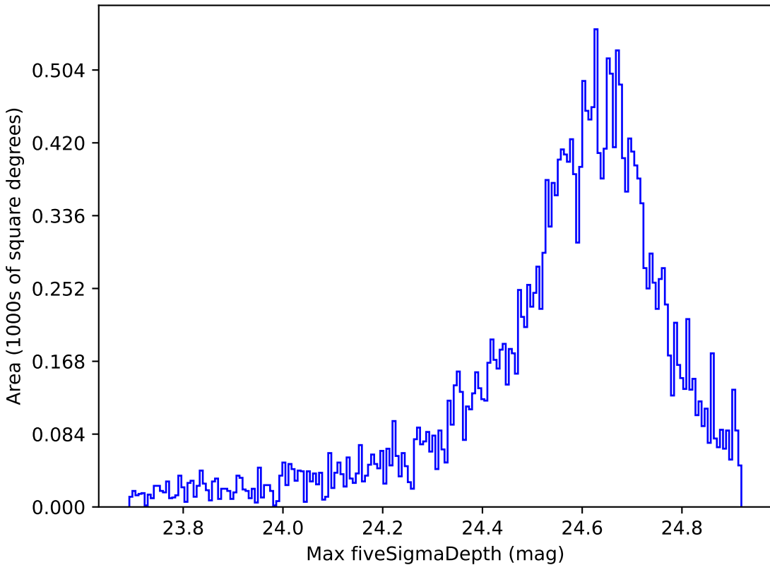
all_long_v3.4_10yrs Yr 1 r band: Max fiveSigmaDepth
