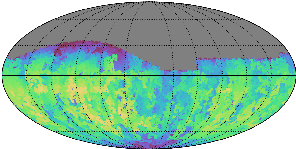
all_long_v3.4_10yrs Yr 1 g band: Max fiveSigmaDepth
