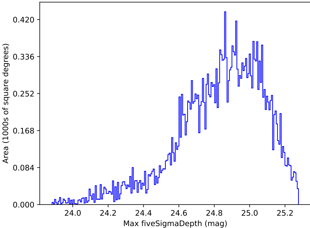
all_long_v3.4_10yrs Yr 1 all bands: Max fiveSigmaDepth
