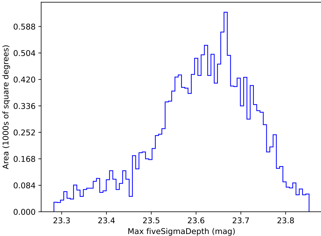
all_long_v3.4_10yrs WFD z band: Max fiveSigmaDepth
