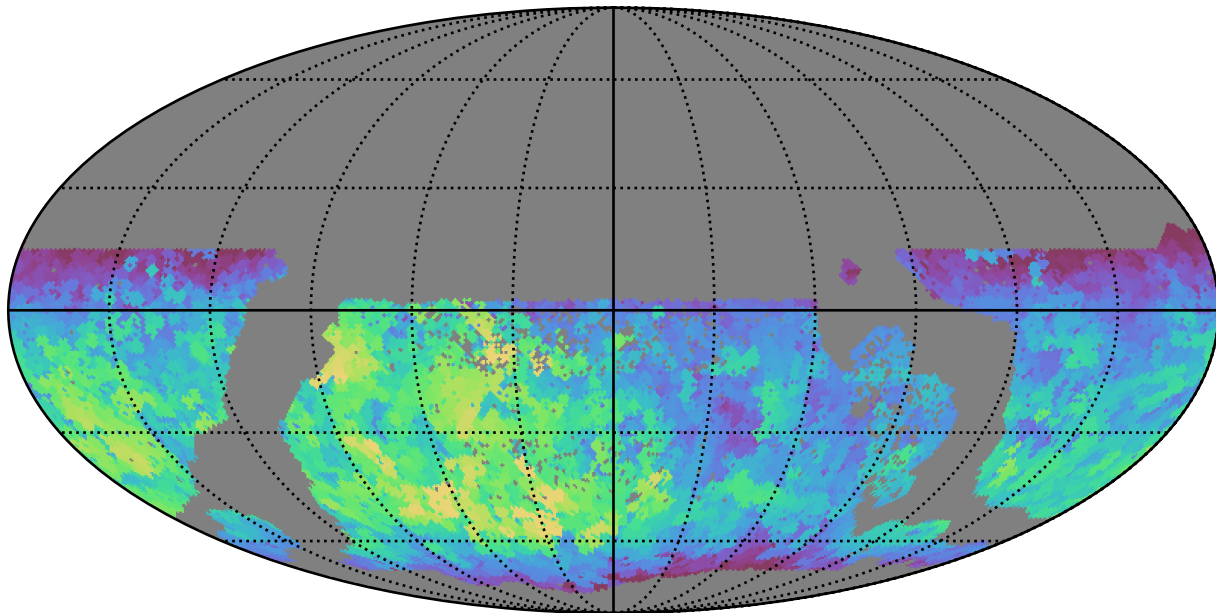
all_long_v3.4_10yrs WFD r band: Max fiveSigmaDepth
