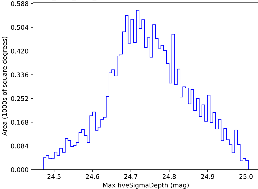
all_long_v3.4_10yrs WFD r band: Max fiveSigmaDepth
