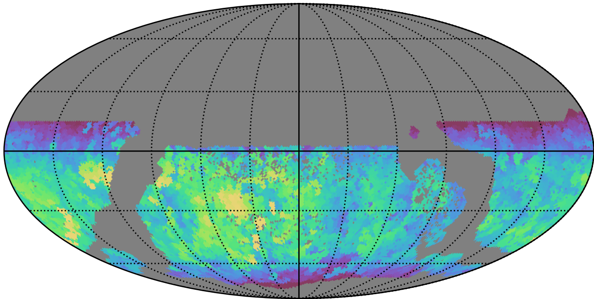
all_long_v3.4_10yrs WFD i band: Max fiveSigmaDepth
