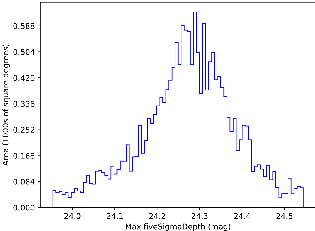
all_long_v3.4_10yrs WFD i band: Max fiveSigmaDepth
