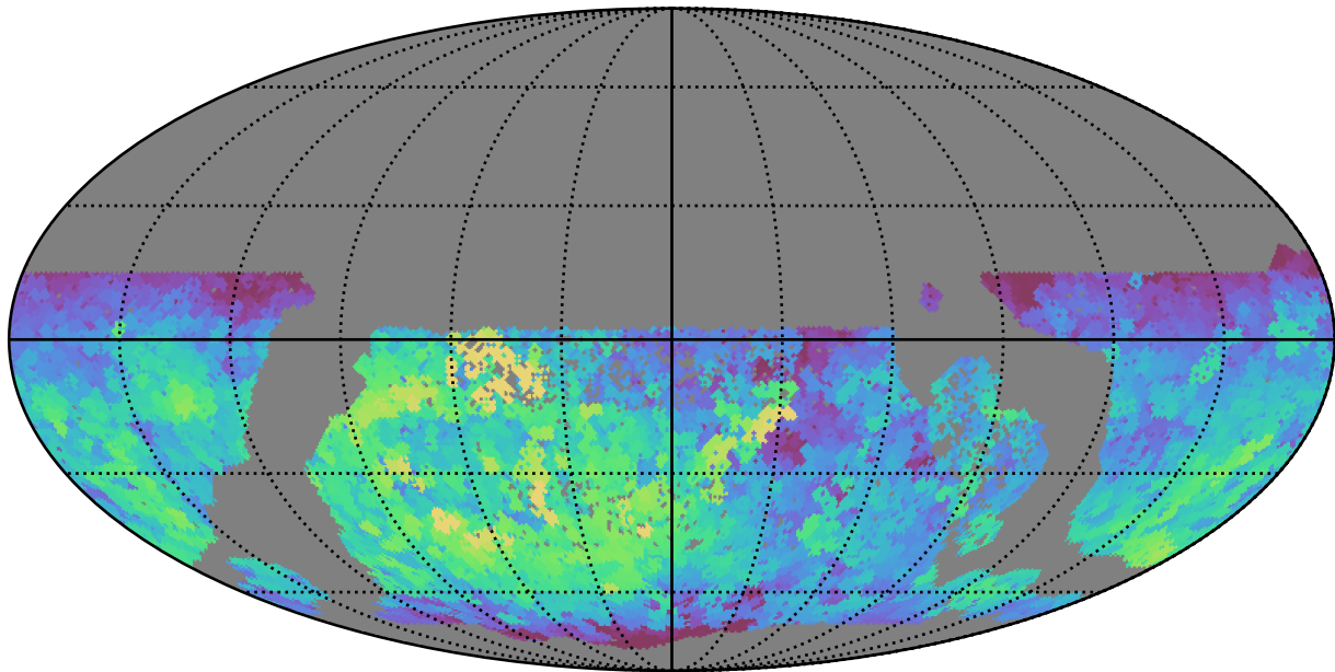
all_long_v3.4_10yrs WFD g band: Max fiveSigmaDepth
