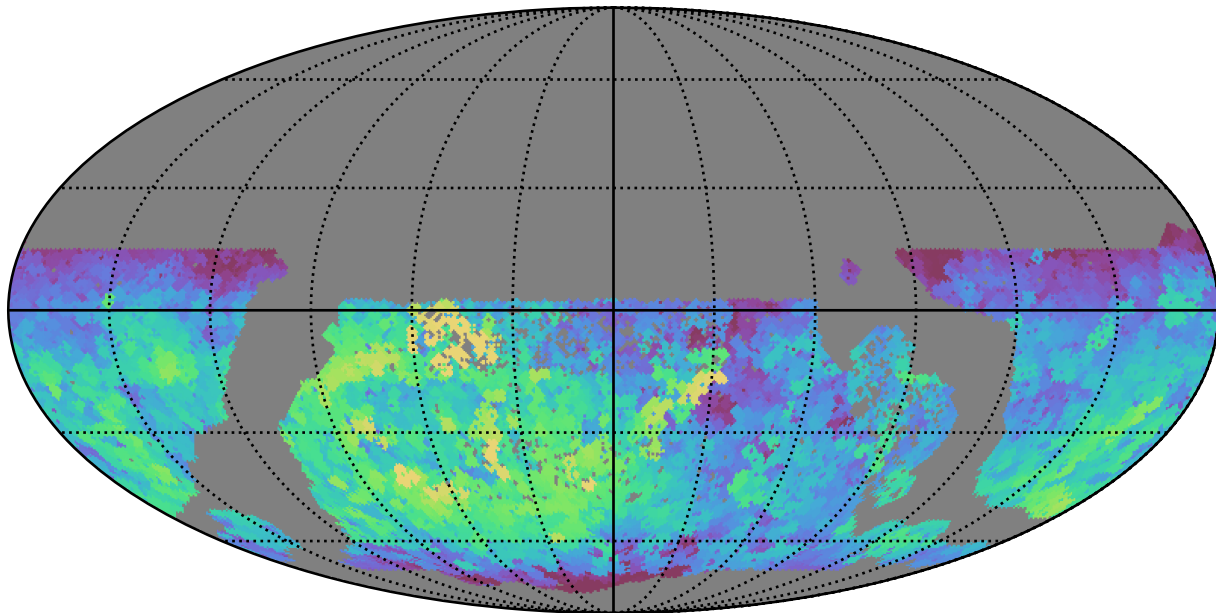
all_long_v3.4_10yrs WFD all bands: Max fiveSigmaDepth
