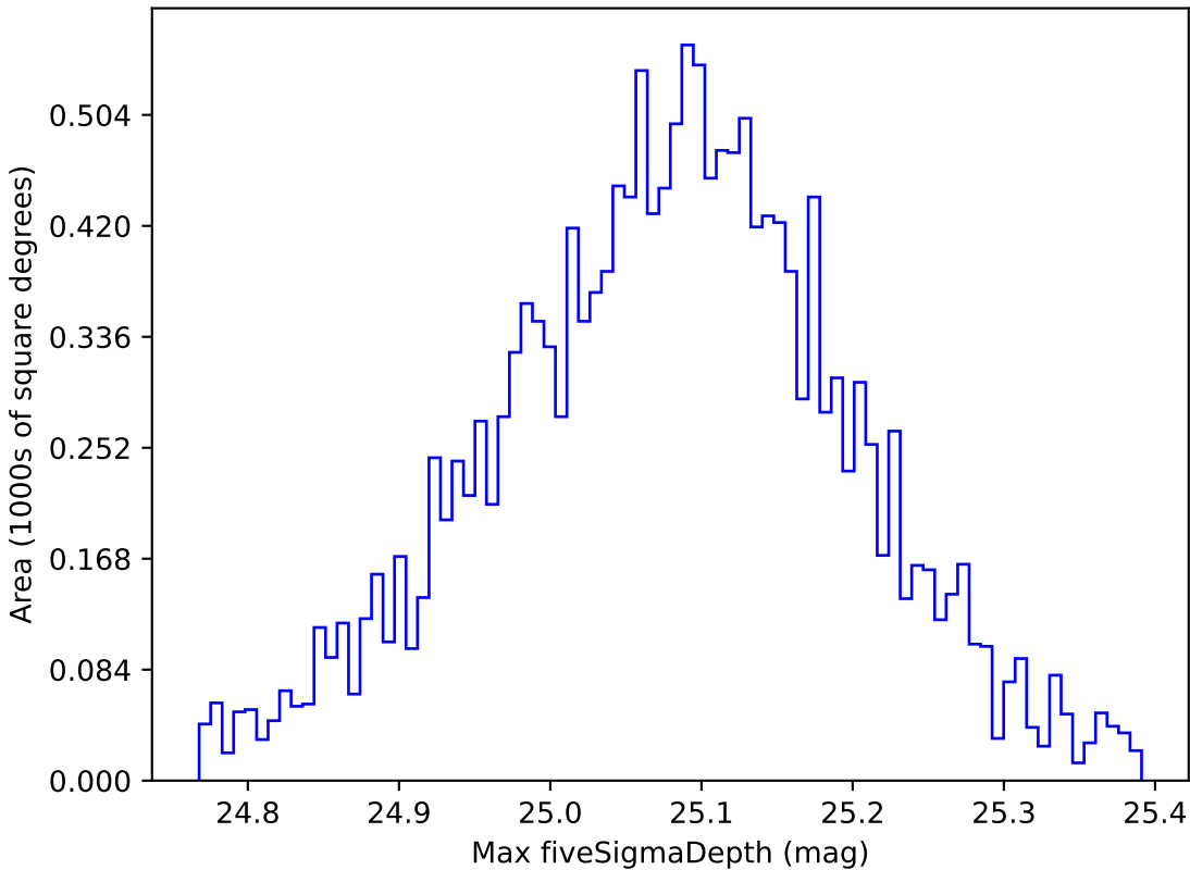
all_long_v3.4_10yrs WFD all bands: Max fiveSigmaDepth
