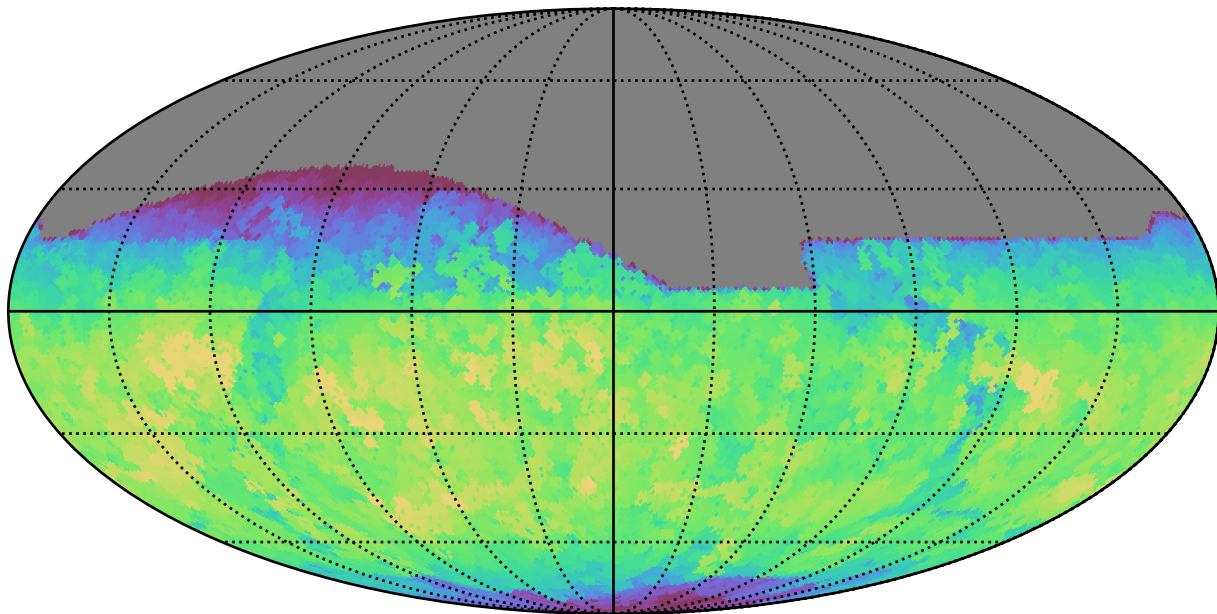
all_long_v3.4_10yrs All sky z band: Max fiveSigmaDepth
