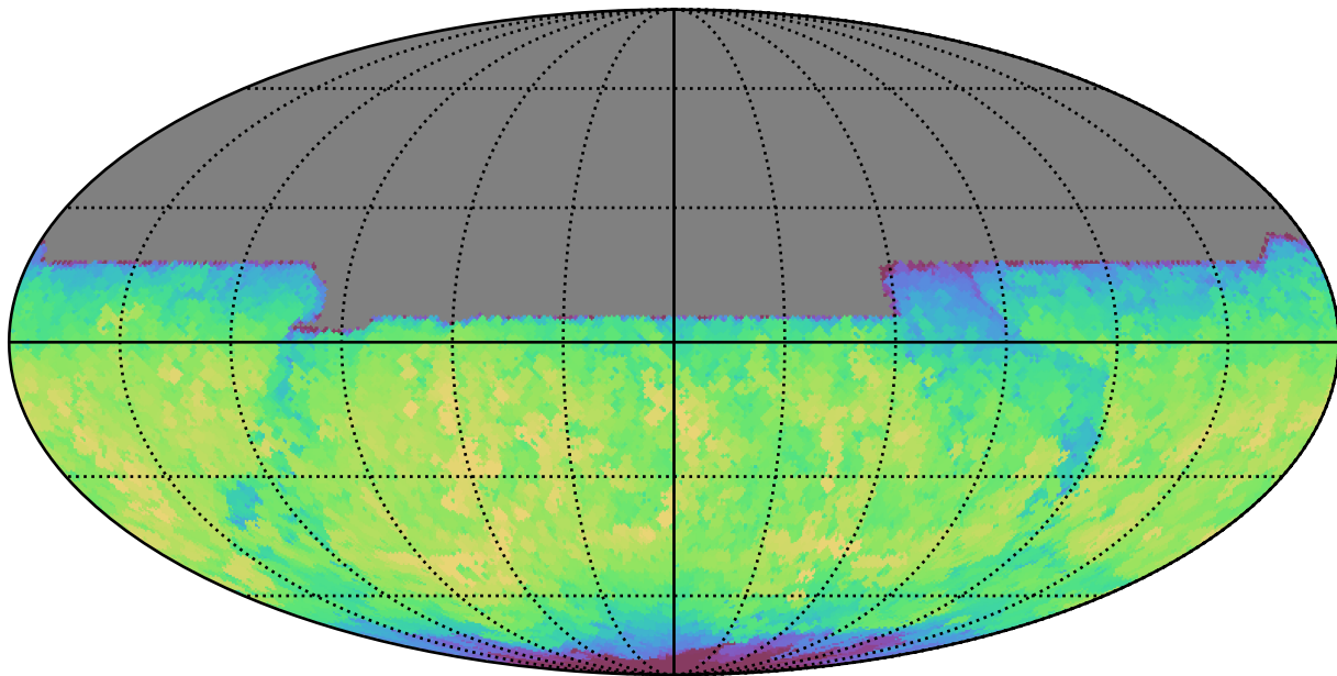
all_long_v3.4_10yrs All sky y band: Max fiveSigmaDepth
