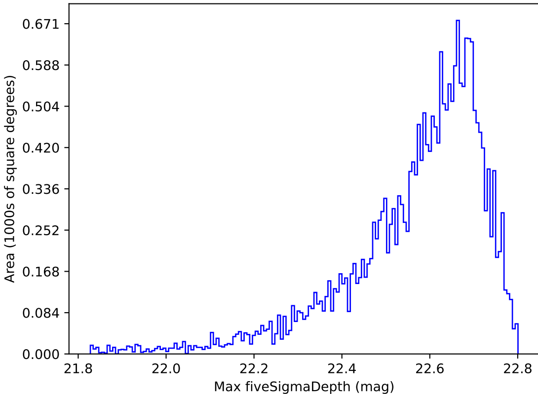
all_long_v3.4_10yrs All sky y band: Max fiveSigmaDepth
