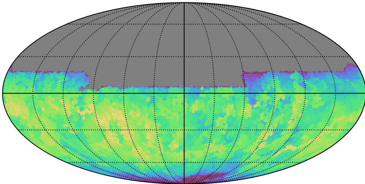
all_long_v3.4_10yrs All sky u band: Max fiveSigmaDepth
