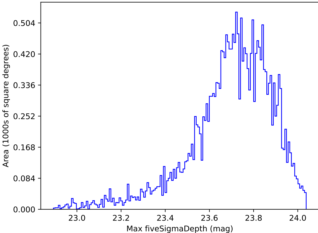
all_long_v3.4_10yrs All sky u band: Max fiveSigmaDepth
