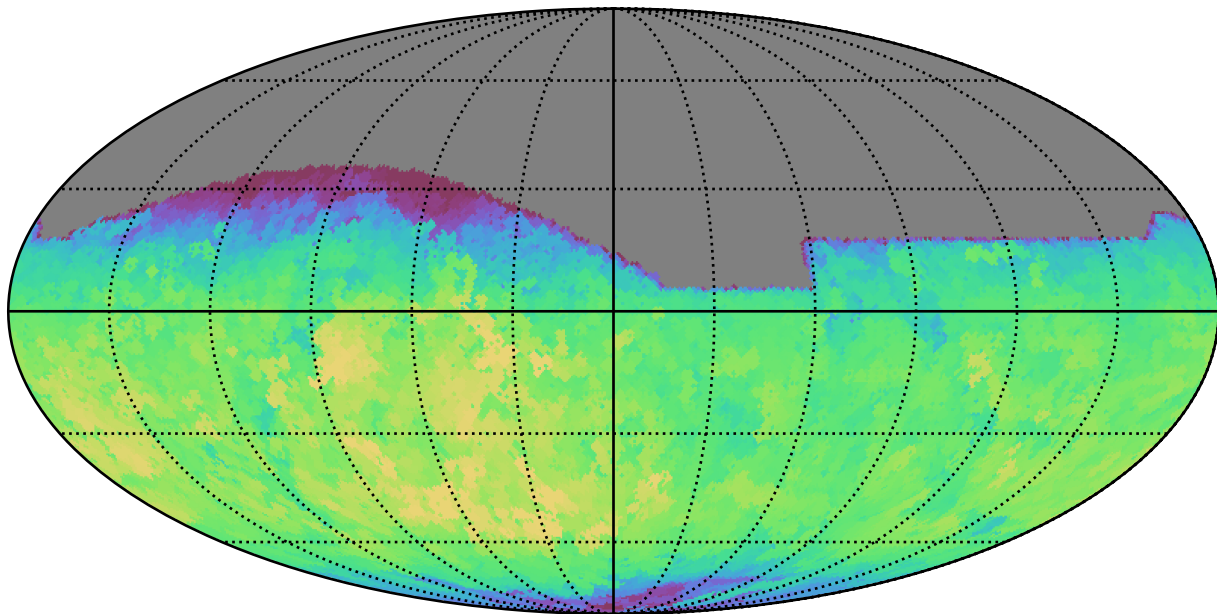
all_long_v3.4_10yrs All sky r band: Max fiveSigmaDepth
