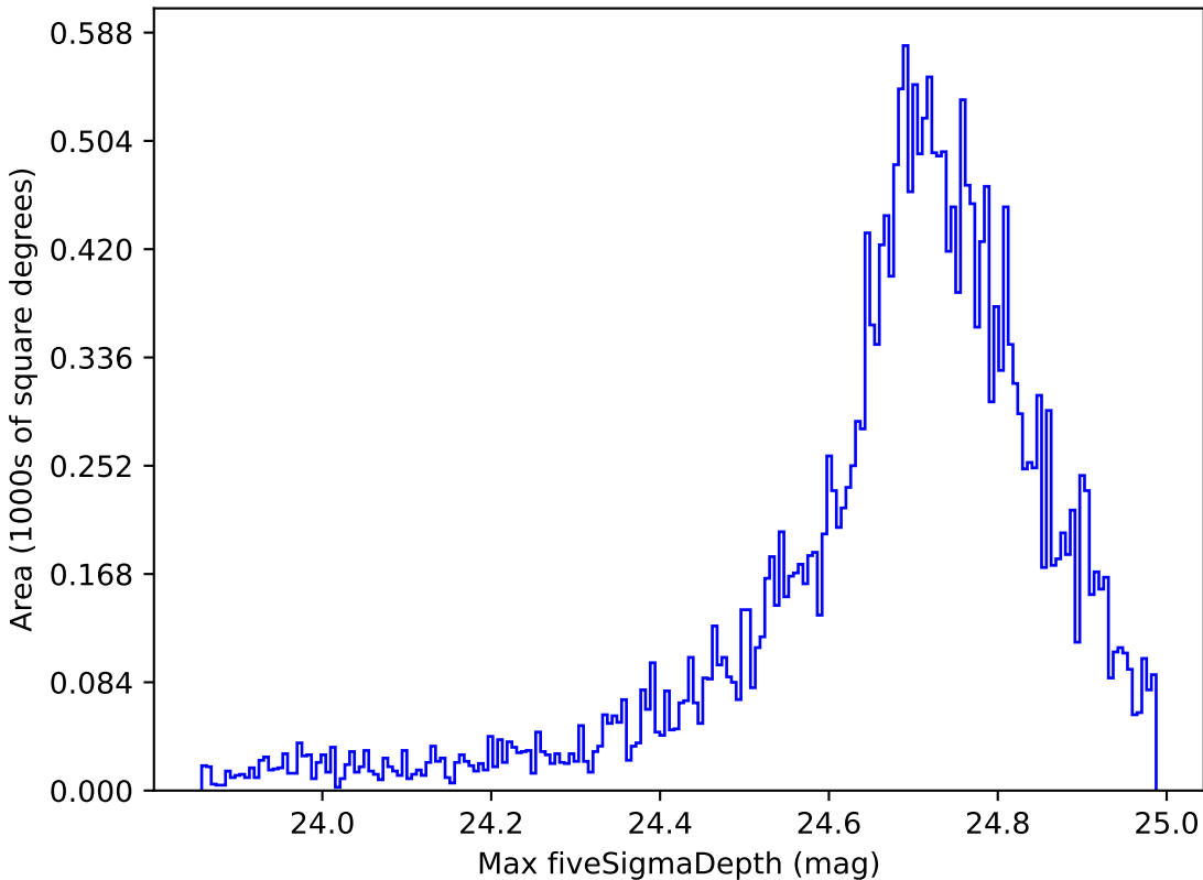
all_long_v3.4_10yrs All sky r band: Max fiveSigmaDepth
