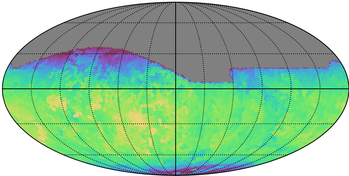
all_long_v3.4_10yrs All sky i band: Max fiveSigmaDepth
