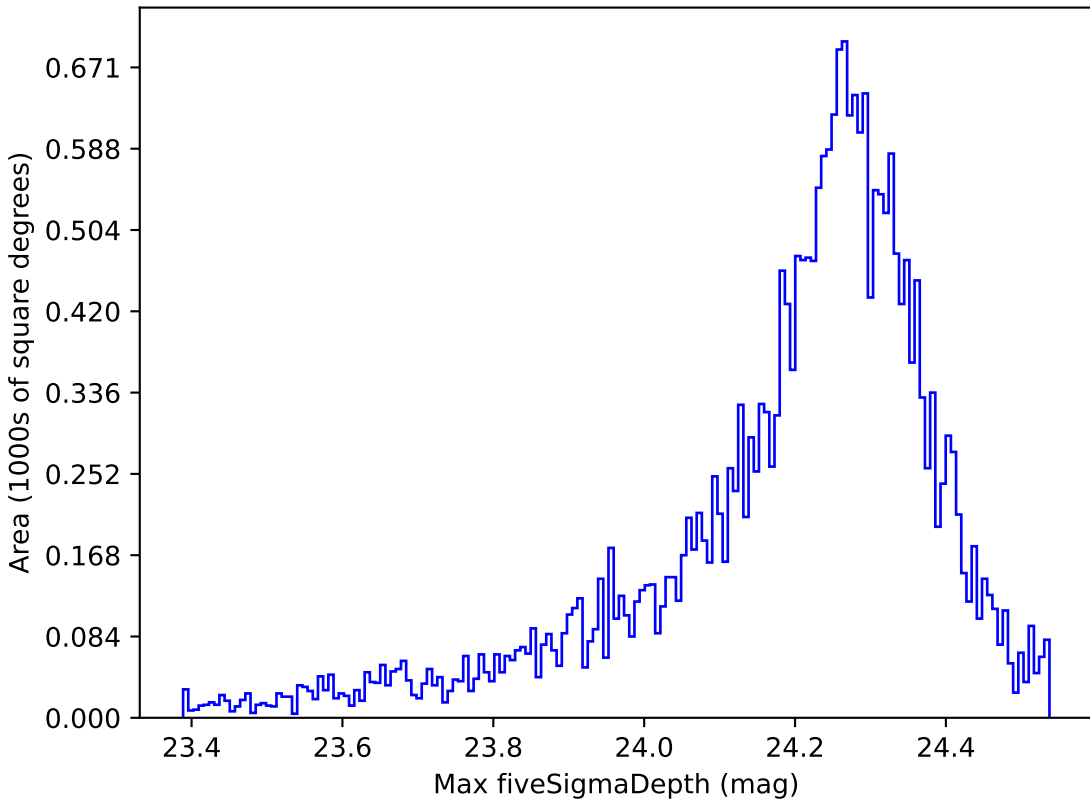
all_long_v3.4_10yrs All sky i band: Max fiveSigmaDepth
