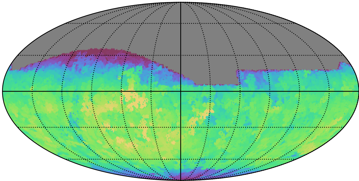
all_long_v3.4_10yrs All sky g band: Max fiveSigmaDepth
