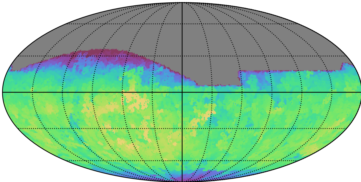
all_long_v3.4_10yrs All sky all bands: Max fiveSigmaDepth
