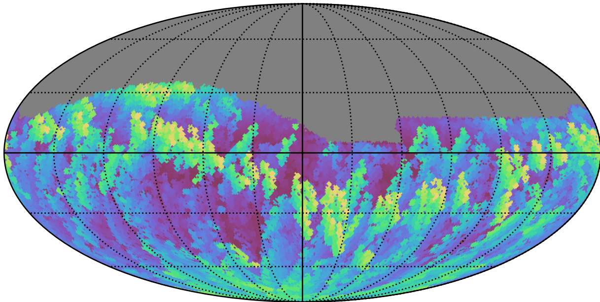
all_long_v3.4_10yrs Yr 1 z band: Max airmass
