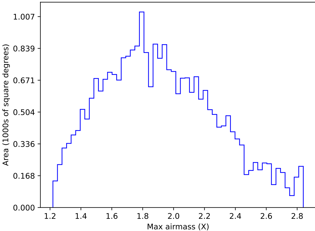
all_long_v3.4_10yrs Yr 1 z band: Max airmass
