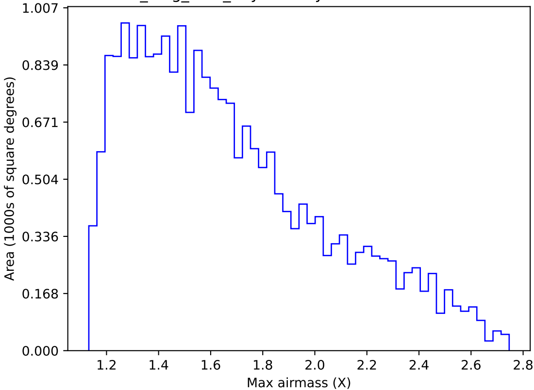
all_long_v3.4_10yrs Yr 1 y band: Max airmass
